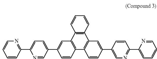
[Chemical Formula 8]
