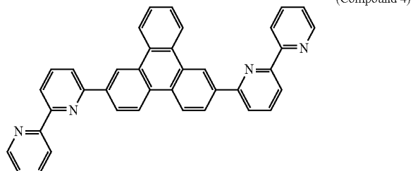
[Chemical Formula 9]
