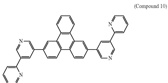
[Chemical Formula 15]
