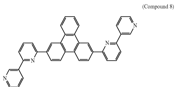
[Chemical Formula 13]
