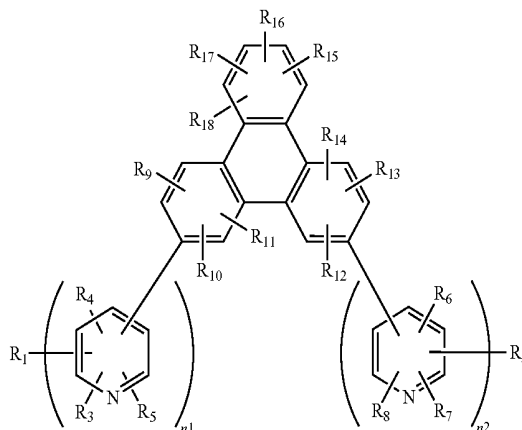
[Chemical Formula 4]
