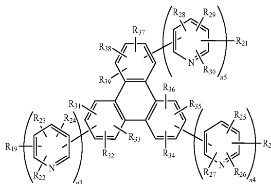
[Chemical Formula 2]
