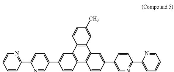
[Chemical Formula 10]
