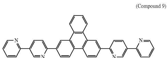
[Chemical Formula 14]
