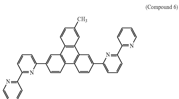
[Chemical Formula 11]
