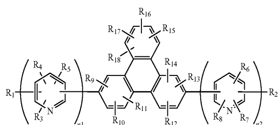
[Chemical Formula 3]
