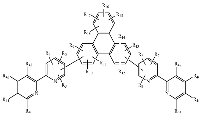
[Chemical Formula 5]
