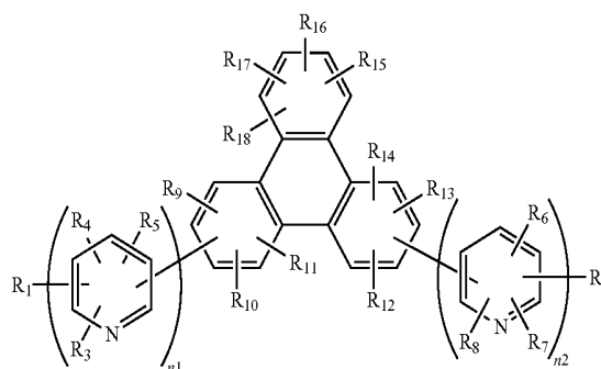
[Chemical Formula 1]
