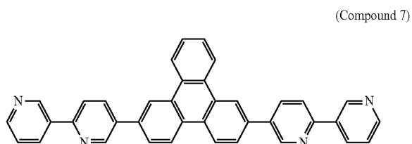
[Chemical Formula 12]
