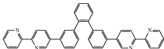
(comparative compound 1)
