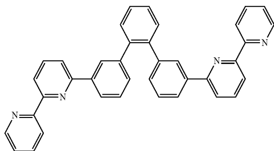
(comparative compound 2)
